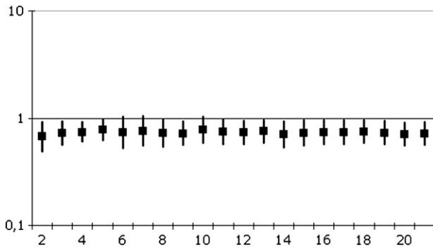
Figure 2. Indicates that all but 3 of 20 possible cut-off values lead to a significant effect if we consider all higher quality trials. The exceptions are n = 144 (including 6 trials), n = 122 (7 trials) and n = 98 (10 trials). If the cut-off point is below n = 98 the pooled results of higher quality studies is consistently statistically significant.
